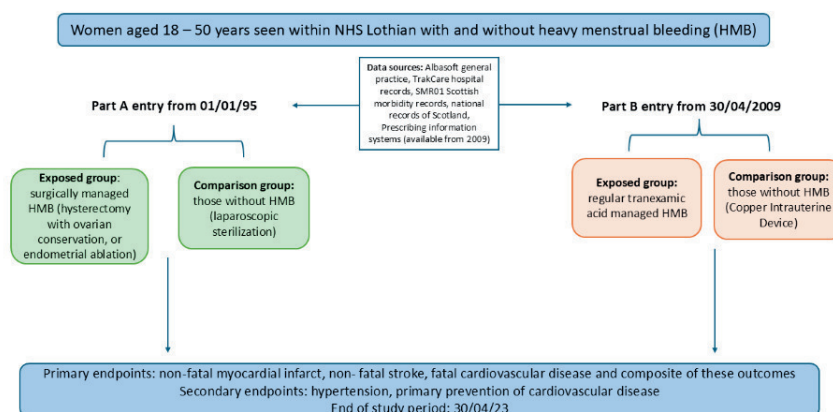
Figure 1 study flowchart
