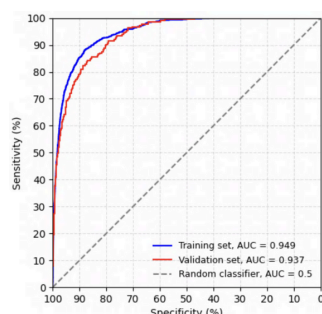
Figure 1: ROC Curves for training and validation sets
